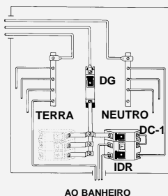
(B) FASE-NEUTRO
